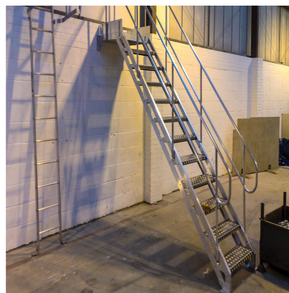
Protection Staircase, Custom Tread Plates NY
