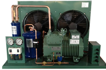
Condensing Units
