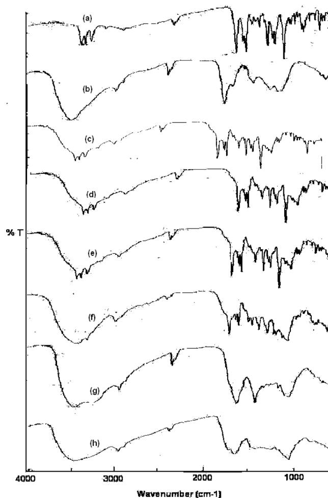
FIGURE 1. FTIR spectra of FSM-FA system prepared by different techniques: (a) FSM alone, (b) FA, (c) 1:1 physical mixture (PM), (d) 1:2 PM, (e) 1:1 solvent evaporation (SE), (f) 1:2 SE, (g) 1:1 freeze dried (FD), and (h) 1:2 FD.
