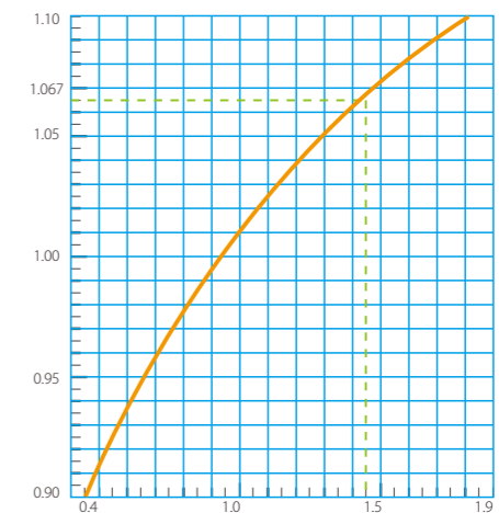
Figure 2 Water velocity correction coefficient F3
