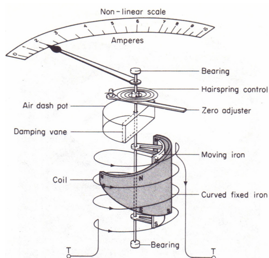
Fig. 39.8. Moving-iron ammeter (improved pattern)
