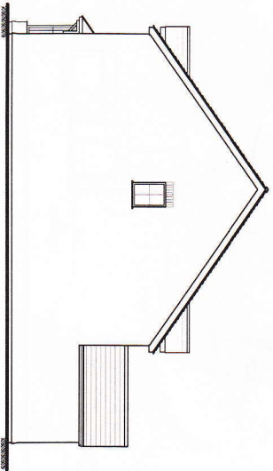
Proposed Right Side Elevation scale 1:100
