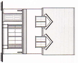
Proposed Front Elevation scale 1:100
