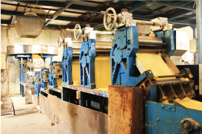
Pressing Process
