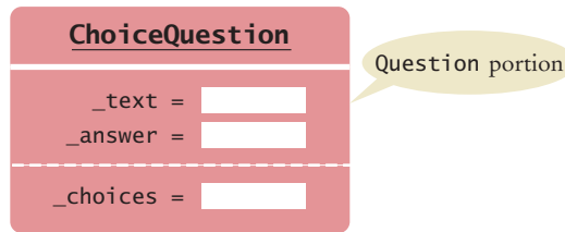
Figure 6 Data Layout of Subclass Object
