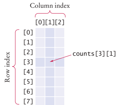
Figure 12 Accessing an Element in a Table
