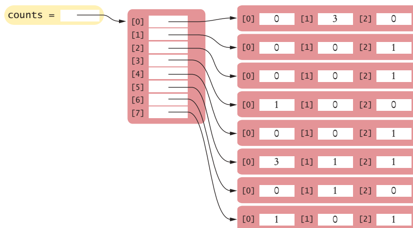
Figure 11 A Table Created Using a List of Lists
