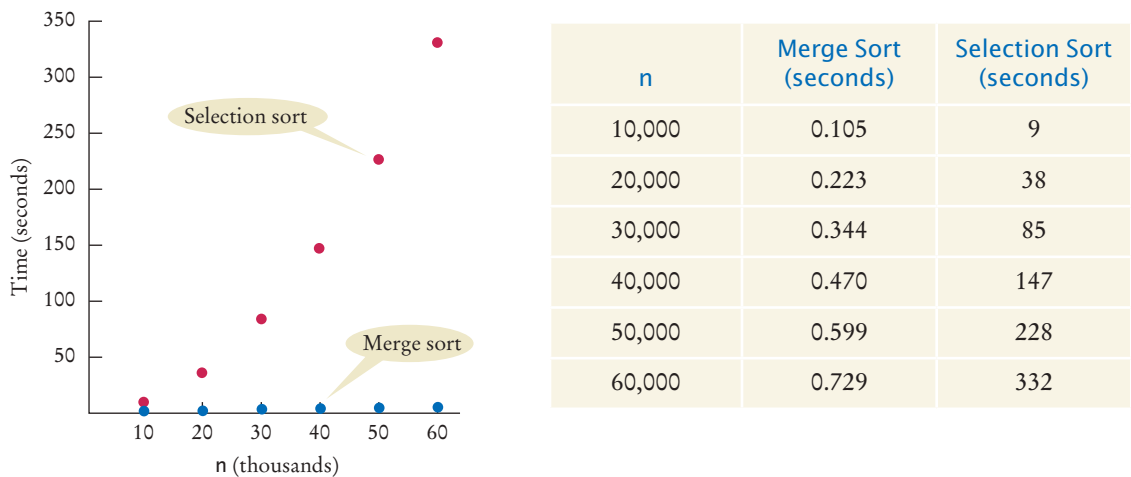
Figure 2 Time Taken by Selection Sort
