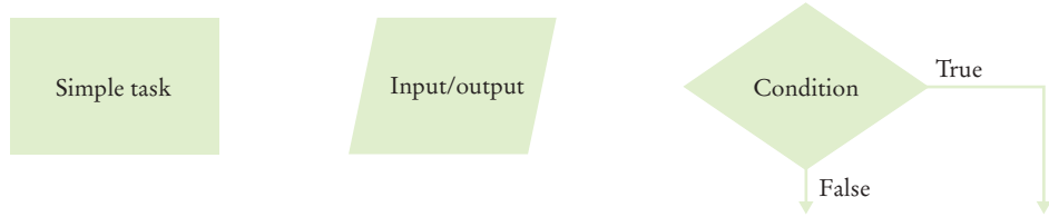
Figure 5 Flowchart Elements
