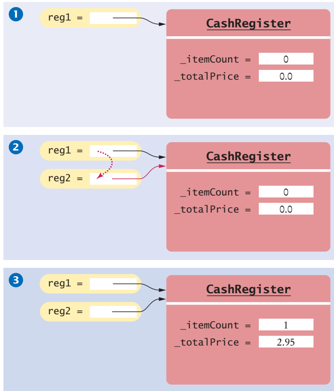
Figure 7 Copying Object References
