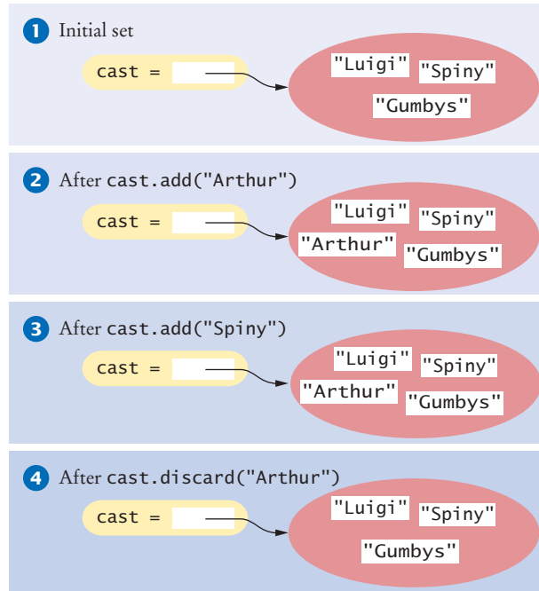
Figure 2 Adding and Discarding Set Elements
