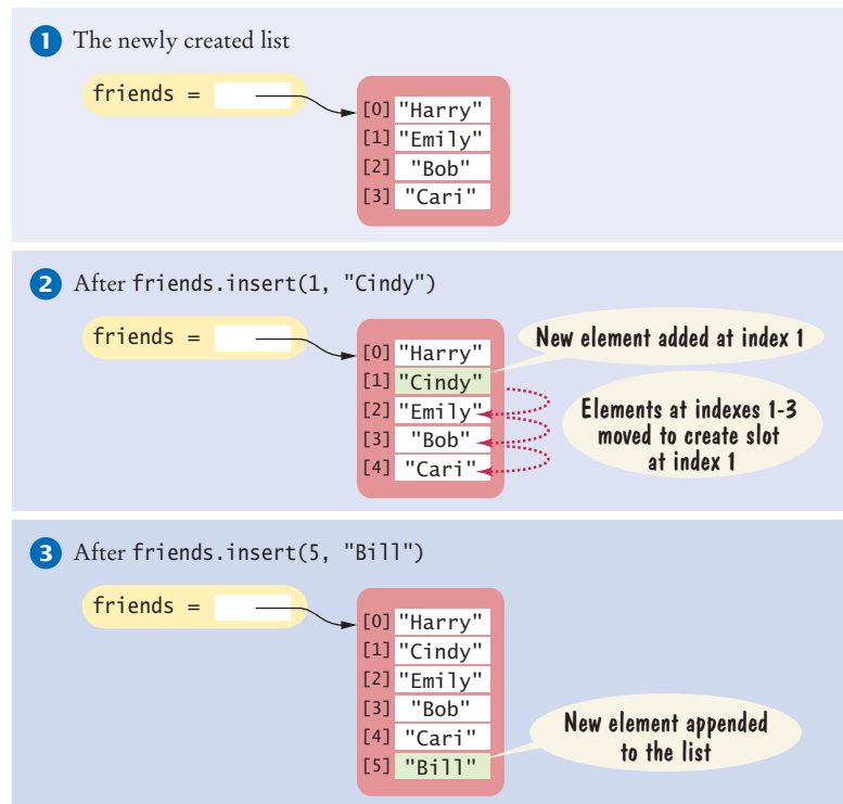
Figure 4 Inserting Elements into a List
