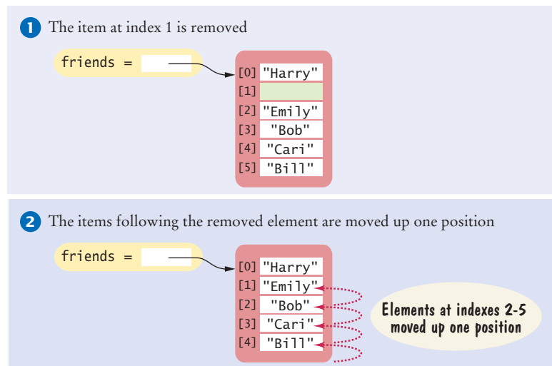
Figure 5 Removing an Element from a List
