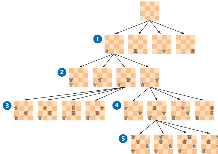
Figure 3 Backtracking in the Four Queens Problem
