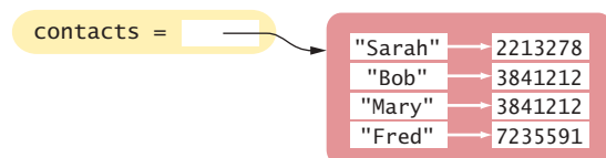
Figure 8 A Dictionary with Four Entries
