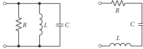
(a) Parallel resonant circuit
