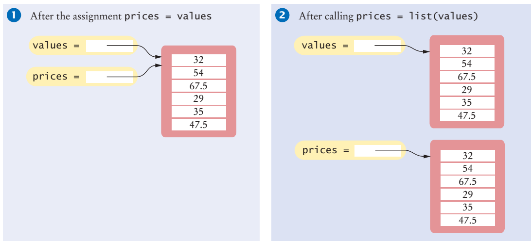
Figure 6 Copying a List Reference versus Copying a List
