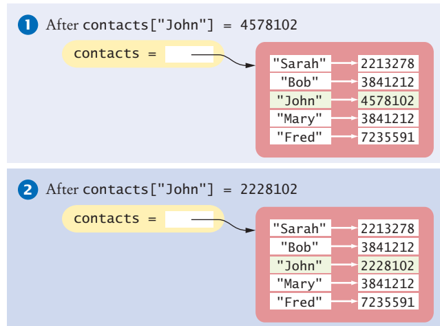
Figure 9 Adding and Modifying Dictionary Entries
