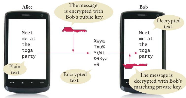
Public-Key Encryption
