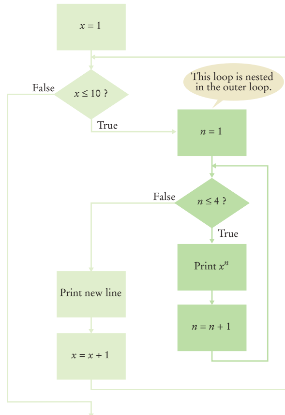
Figure 5 Flowchart of a Nested Loop
