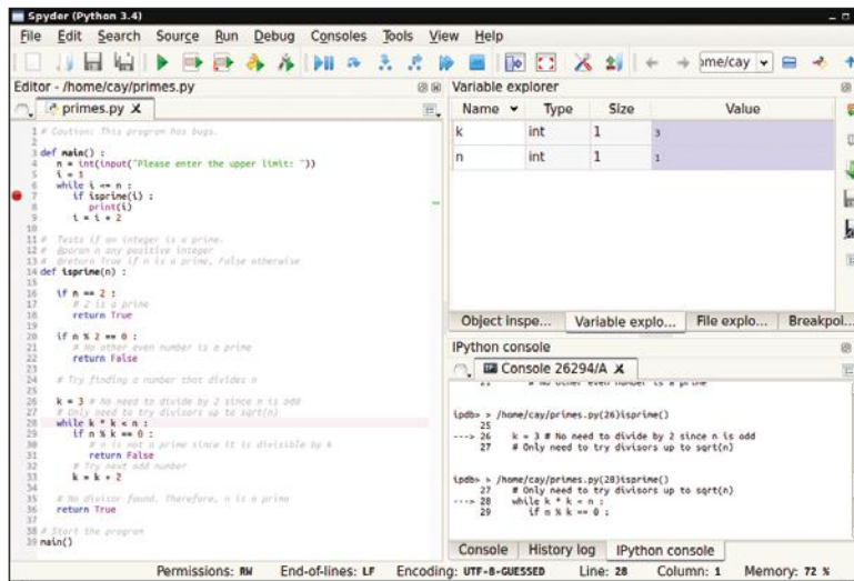
Figure 6 The Debuggers of Spyder, PyDev, and PyCharm
