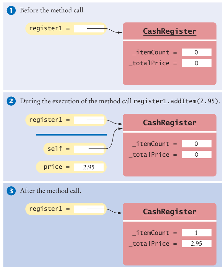
Figure 4 Assignment of the self Reference
