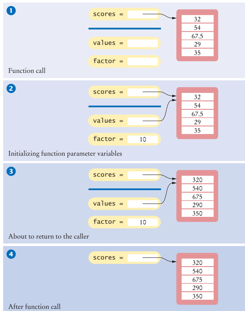
Figure 8 Trace of Call to the multiply Function
