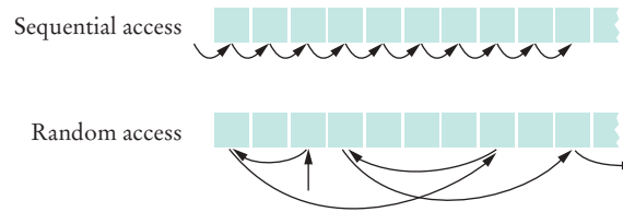
Figure 2 Sequential and Random Access
