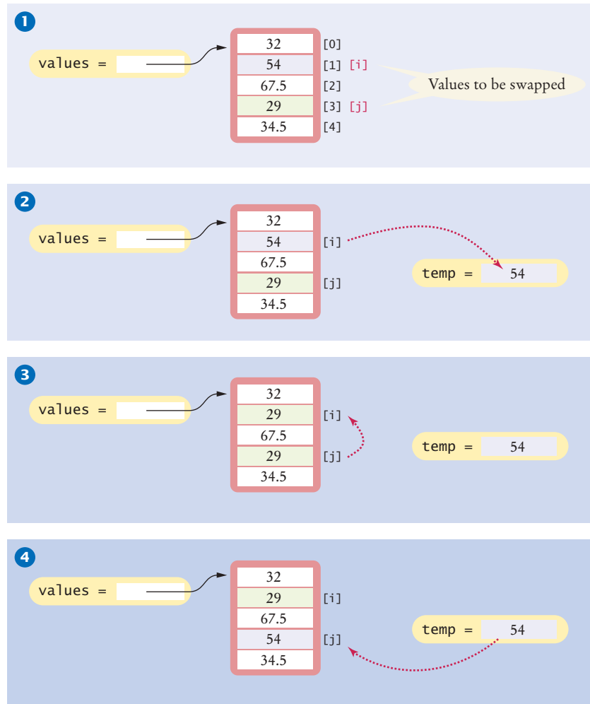
Figure 7 Swapping List Elements
