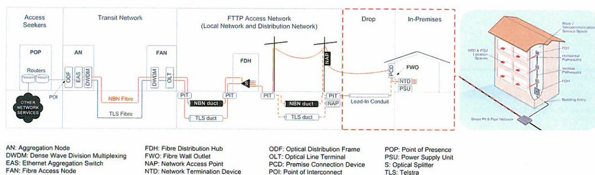
Exhibit 11-4: Diagram of a Multiple Dwelling Unit (MDU) in the Fibre Access Network
