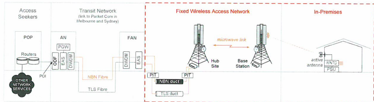
Exhibit 13-1: Overview of Fixed Wireless & Satellite Networks
