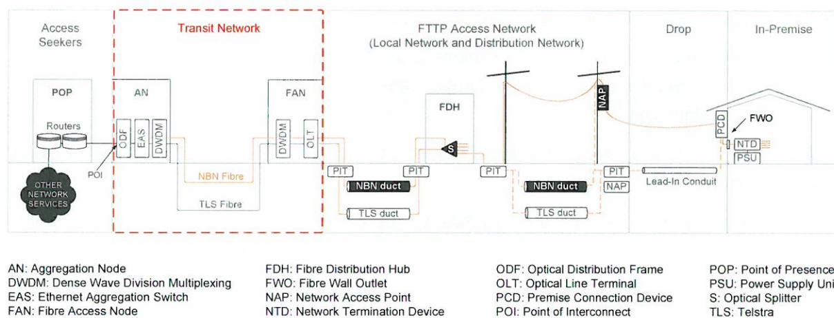
Exhibit 9-1: Overview of the Transit Network
