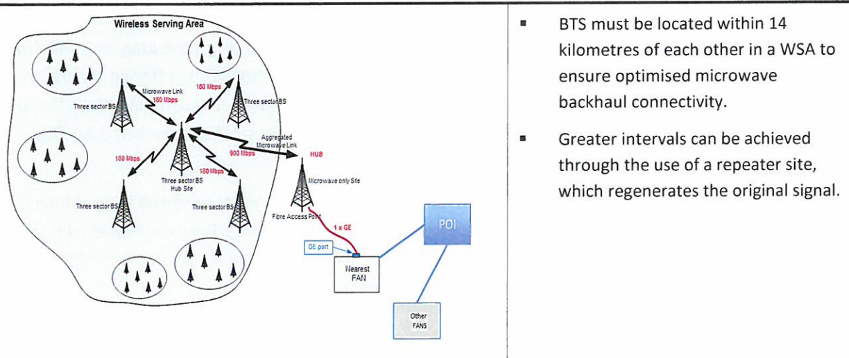
Exhibit 13-4: Typical Wireless Cluster
