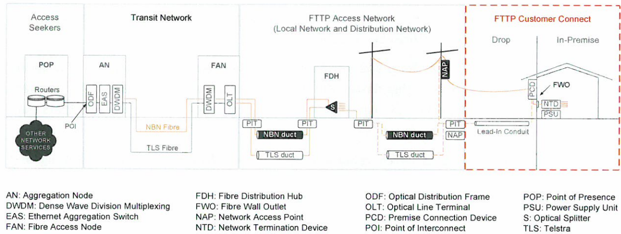
Exhibit 11-1: Overview of FTTP Customer Connect
