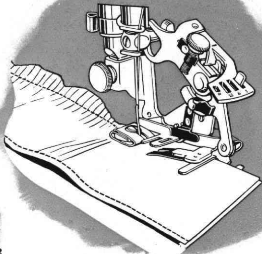
Fig. 65. Making a Ruffle and Attaching it in One Operation
