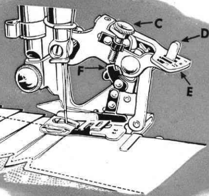
Fig. 70. Plaiting with Ruffler
