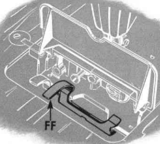
Fig. 2. Showing Latch for Releasing Machine from Cabinet
