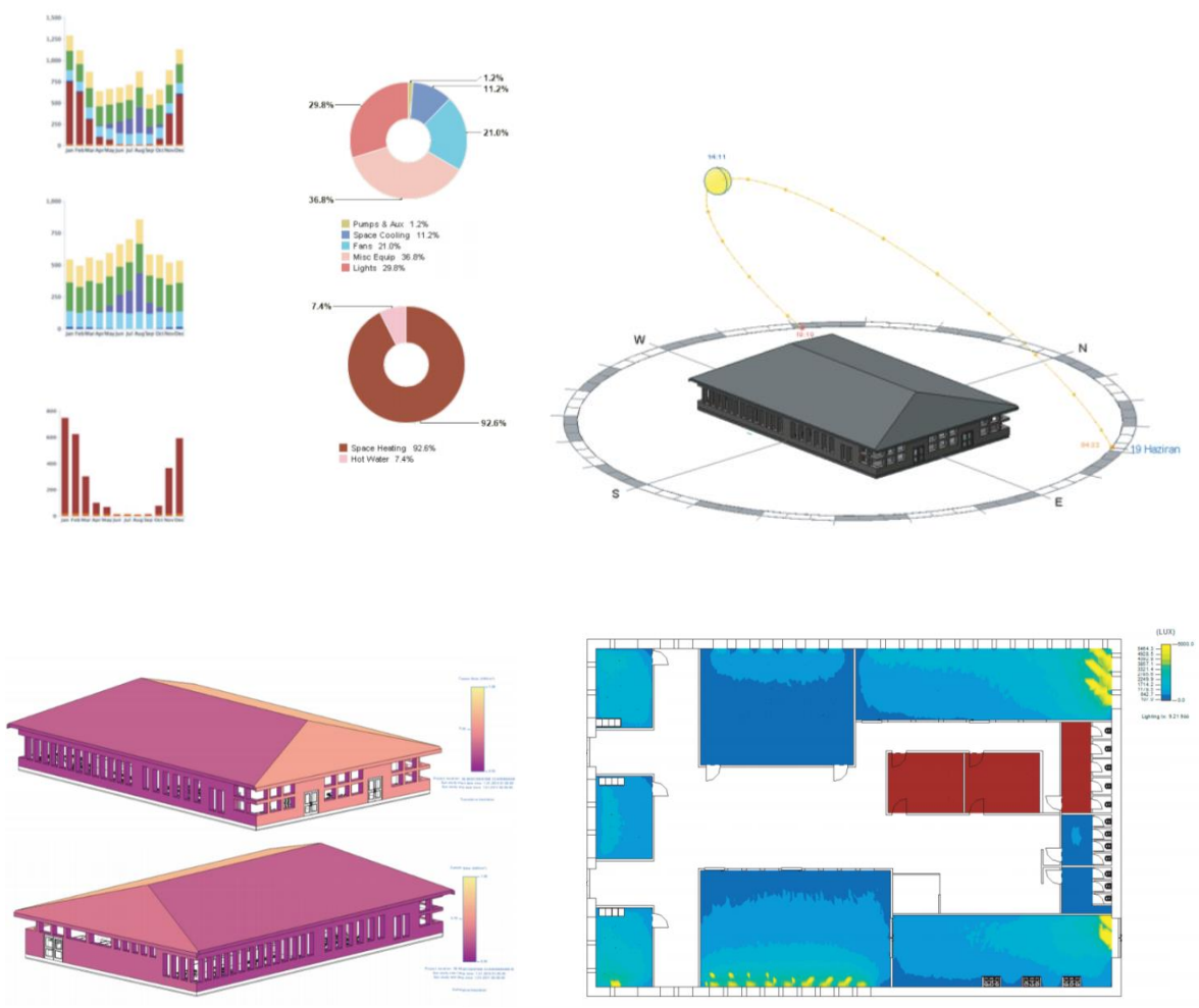
Fig.2: First energy analysis graphics from the generated BIM model a primary school project by Nursima Zengin-ADPR IV
