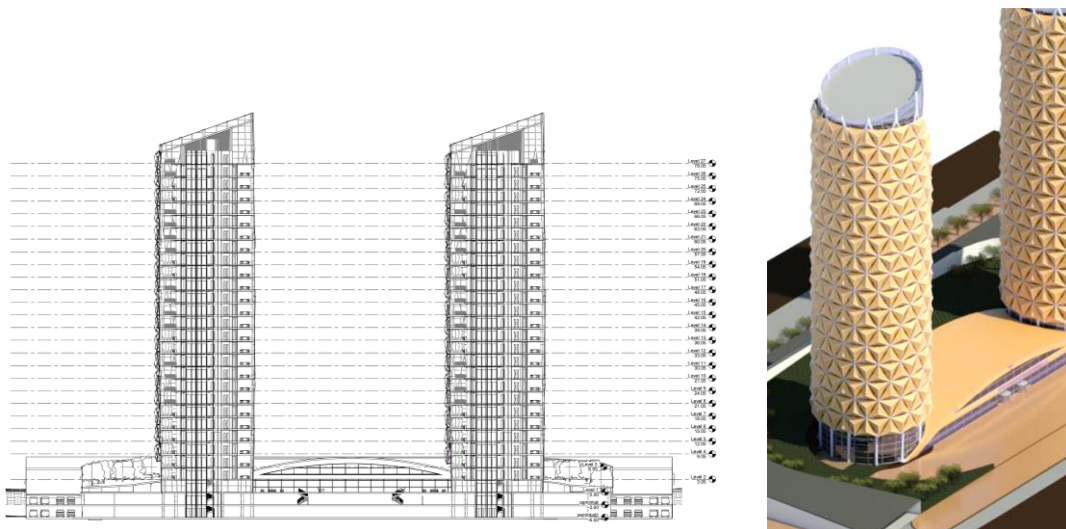
Fig.1: Section and model views from the generated BIM model of Al Bahar Towers by Azime Ecrin Akkaya-ADPR III
