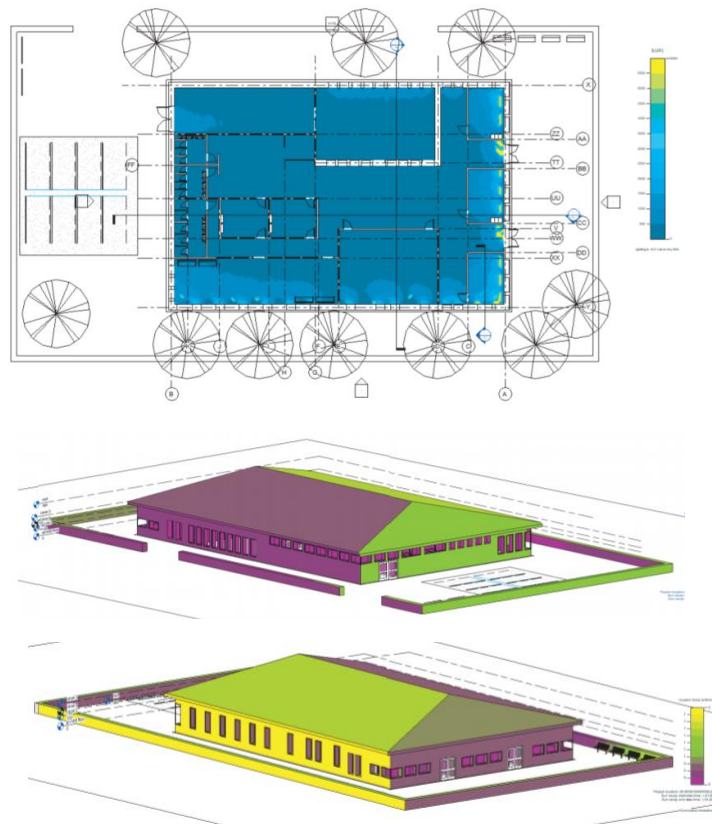
Fig.3: Last energy analysis graphics from the generated BIM model a primary school project by Nursima Zengin-ADPR IV
