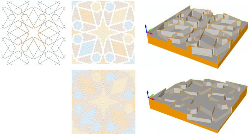
Figure 2: Three stages of the model generation (from left): Generating a 2d pattern, generating 2 1/2 axis toolpath variations, simulating milled model variations (Image courtesy: Şeref Atilla Gürbüz)
