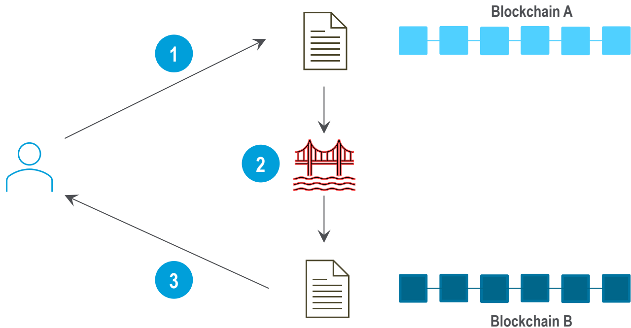
Figure 31. Lock-and-Mint Bridges
