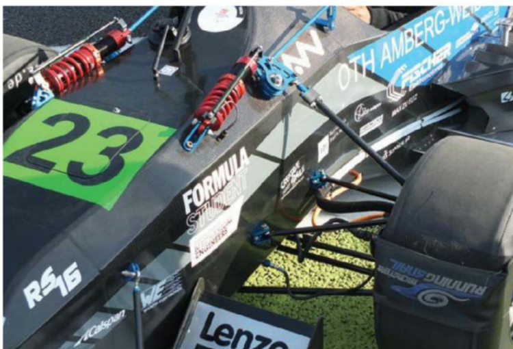
The Amberg-Weiden entry used a quite simple and certainly cost-effective suspension design made from steel, the team's calculations showing that the weight and stiffness ratio was good
