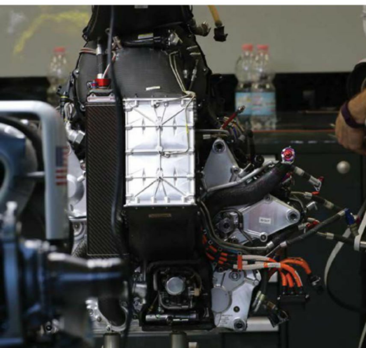
Ferrari power unit in the back of the VF-16. This shows charge air cooler, oil tank and cylinder head. Use of proven technology has helped the Haas team to shine this year
