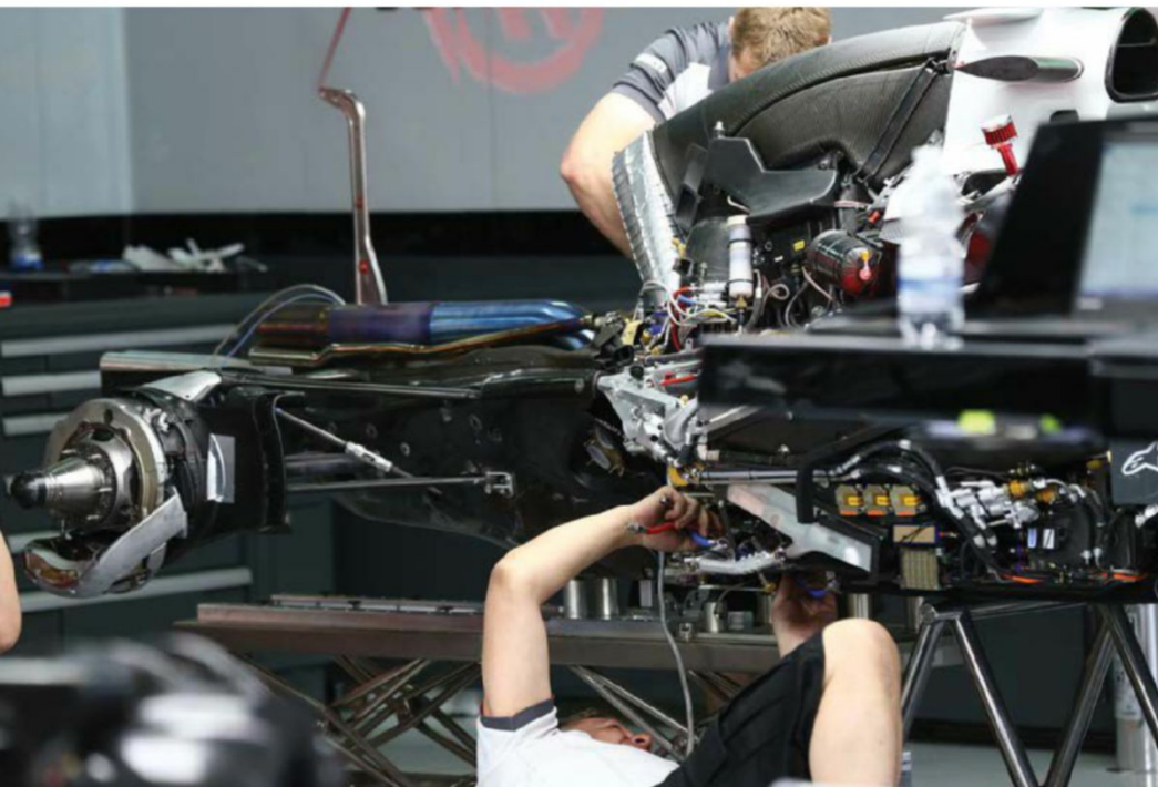
The rear end showing the Ferrari transmission. Haas shares uprights, outboard suspension elements, inboard suspension parts and brake set-up with Ferrari. The VF-16 also has push rod actuated dampers on the front and pull rod on the rear
