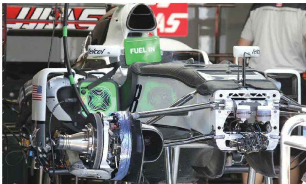
Haas has followed Manor and Red Bull down the machined aluminium front bulkhead route. The team says this does not give it a benefit in terms of chassis stiffness and weight over a carbon example but that it does simplify this area of the car
