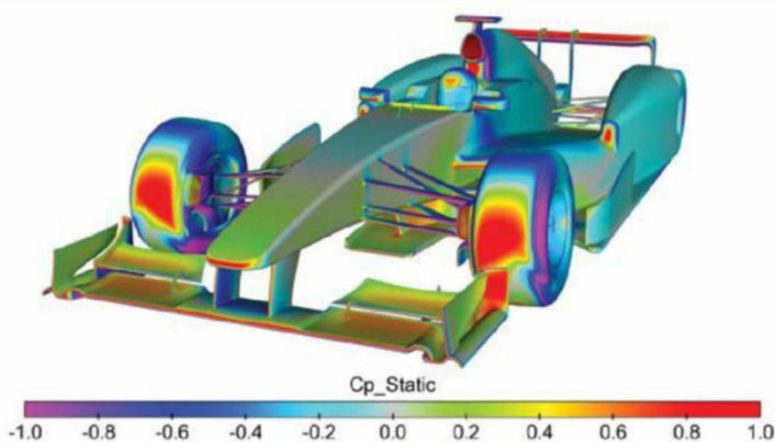
Figure 7: Surface pressure distributions
