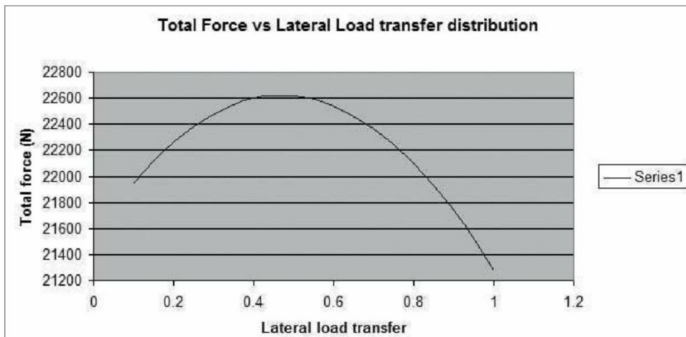
Figure 2: Using sim to reverse-engineer tyres from race data you can plot max lateral grip vs lateral load transfer distribution
