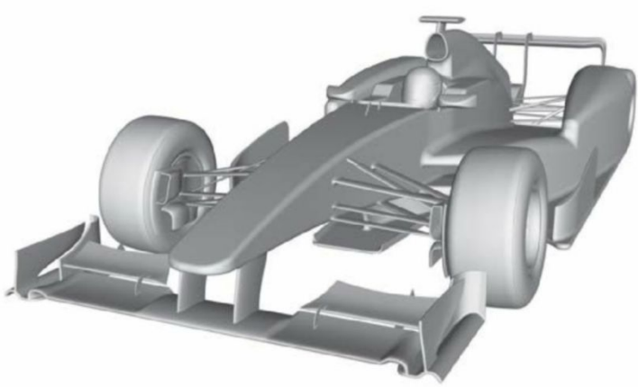
Figure 4: V3 with detuned tunnels, wider body, further detuned wing and wheel fairings
