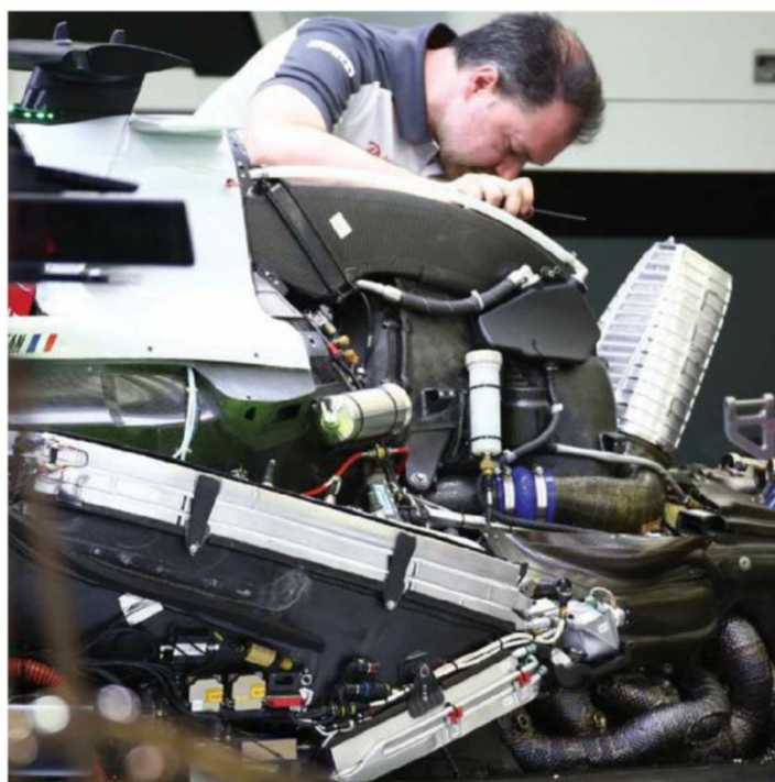
Cooling system uses three coolers stacked on top of each other within each sidepod with a fourth mounted further back forming a V-shape. Again this is similar to Ferrari's system
