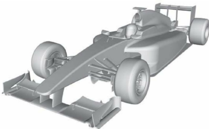
Figure 3: RE 2017 V2 with full underbody tunnels and detuned wings
