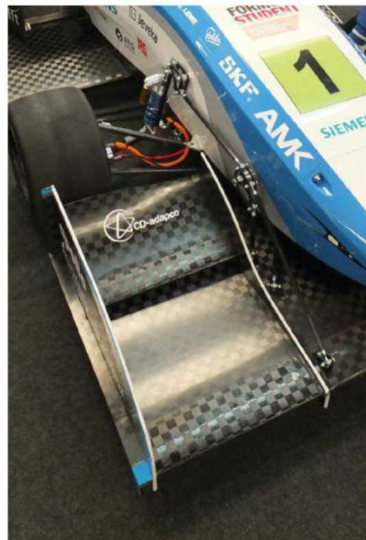
Delft's front wing was twice found to be oversized, firstly during initial tech inspection when it was deemed to be 1mm too high and the team was forced to trim it slightly
