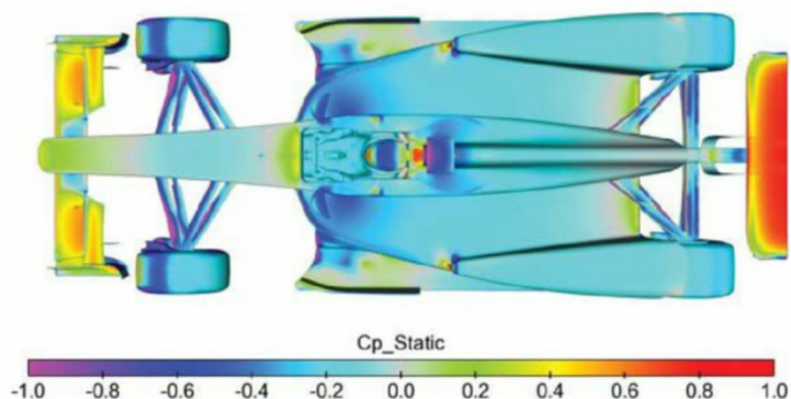
Figure 9: Lift from the upper body surfaces was less than on the V2 model, which helped the total downforce to compare well with our previous designs
