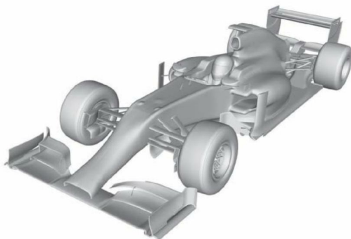
Figure 2: RE's 2017 F1 car with bigger diffuser plus modified and repositioned rear wing
