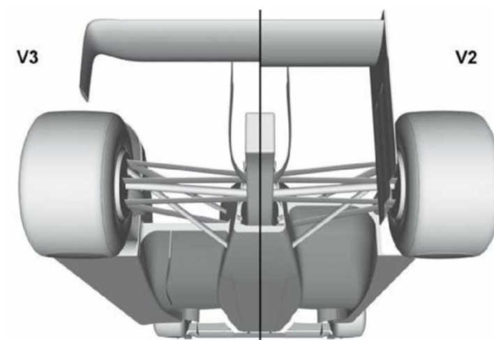
Figure 6: Comparing V2 and V3 from behind and below. The strake in V3's tunnels created a vortex that reduced pressure and increased mass flow for more downforce
