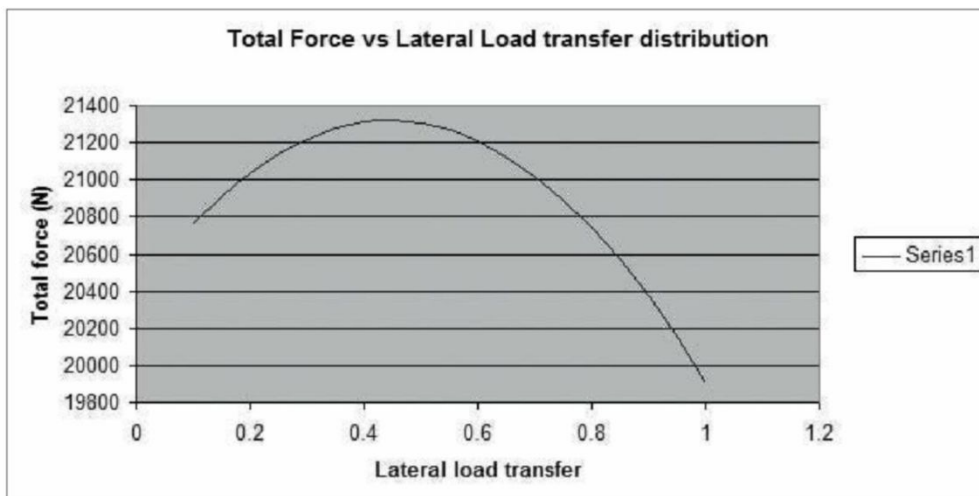
Figure 3: This shows the total force vs lateral load transfer with the rear-wheel-drive racecar model now taken into account
