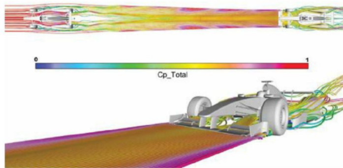
Figure 20: There are less energetic streamlines in the leading car's wake right out to four car lengths, and clearly the air that hits V3's front wing is at reduced total pressure
