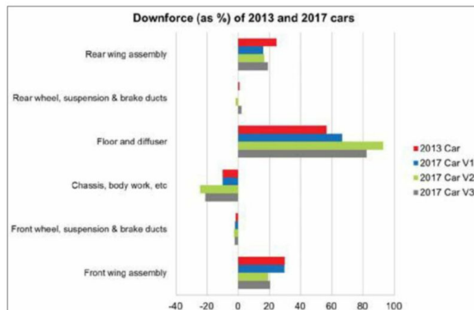
Figure 10: Downforce contributions from the major component groups on our four cars
