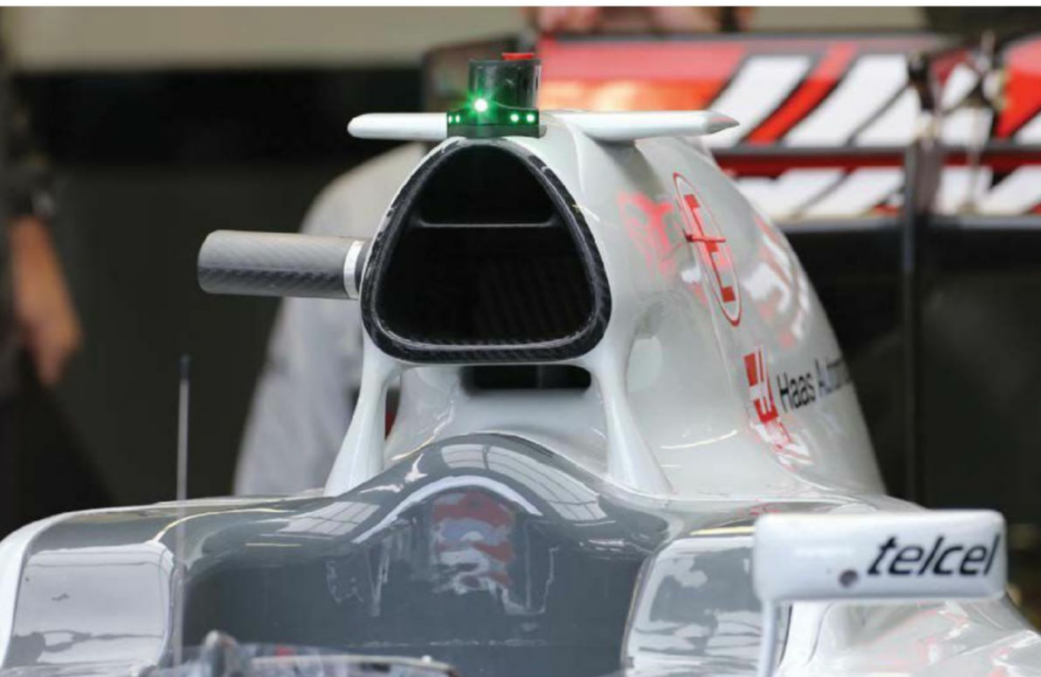
VF-16 has twin sculpted forward roll hoop supports and three separate ducts. The uppermost inlet feeds air to a charge air cooler, the lower one in the hoop provides the combustion air itself, a third below these probably cools electrical components
