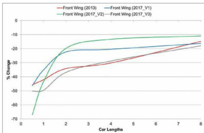
Figure 15: The loss of a larger proportion of the front wing downforce was V3's pitfall
