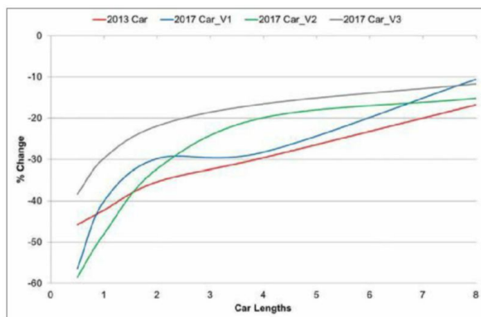
Figure 13: V3 lost much less total downforce when following than the previous designs
