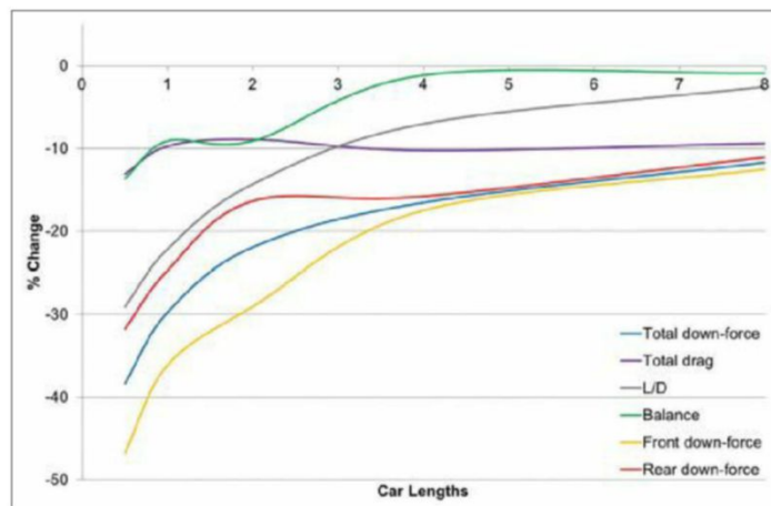
Figure 12: This shows the changes to the principal aerodynamic numbers on the 2017 V3 racecar model when it is following another racecar in a line astern formation
