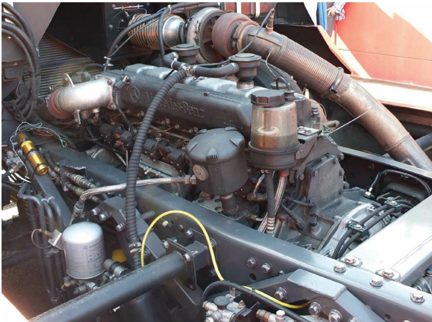
The engines in racing trucks make use of standard parts in the main, up to 90 per cent in fact, although they also use special pistons and injector pumps and optimised turbochargers
