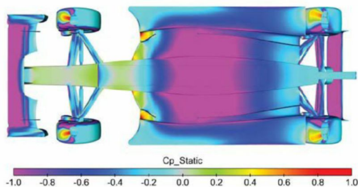
Figure 8: The underbody developed over 80 per cent of the new V3 model's total downforce, which is slightly less than the V2 car model's underbody contribution
