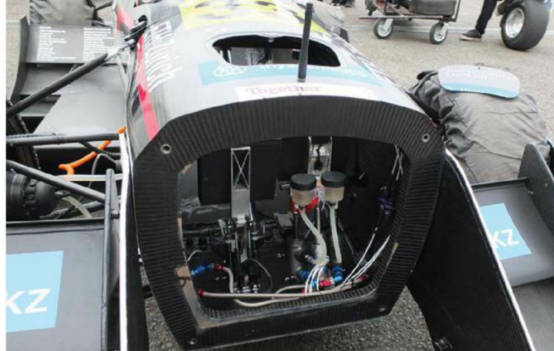
The front bulkhead and the pedal box. Driver aids include traction control for optimal wheel slip plus a torque vectoring system to improve the car's agility on tight FS courses
