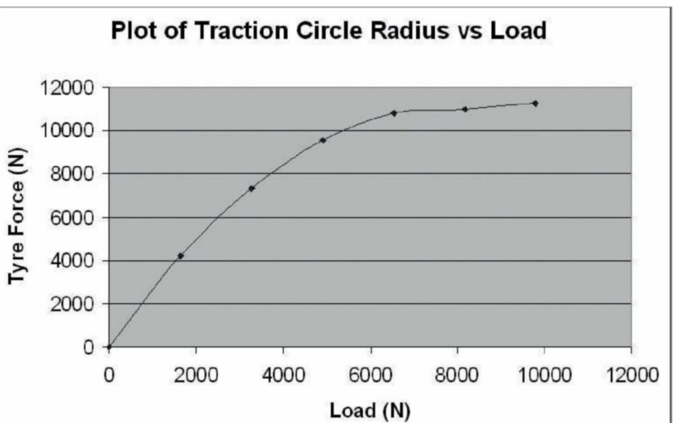
Figure 1: This is a basic second order plot of the traction circle vs load characteristic, showing how load works on the tyres
