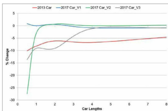
Figure 14: The V3 balance shift was not quite so good at two and one lengths separation
