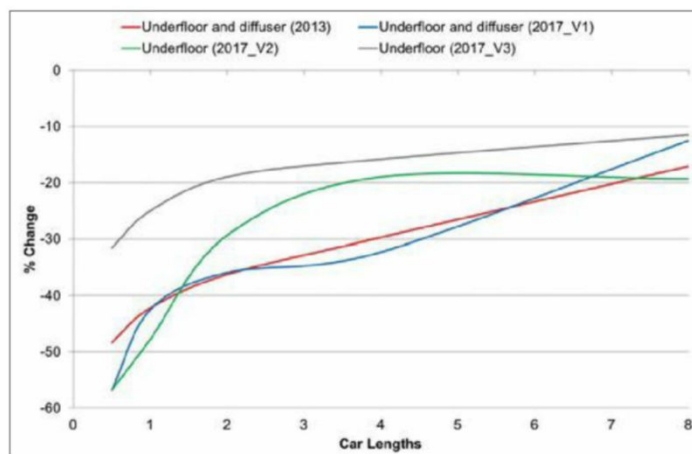
Figure 16: The V3 model's underbody lost far less downforce than the previous designs
