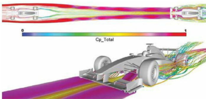
Figure 19: Streamlines coloured by total pressure show how inwash transported energetic tidy air to the following V2 car's front wing at four car lengths separation
