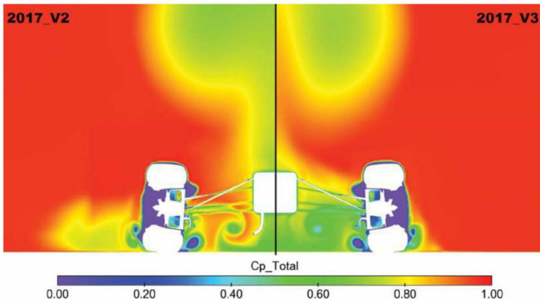
Figure 21: A total pressure slice at the front axle line at four car lengths separation shows that our V3 model's underbody also received less energetic airflow, and yet the underbody performed well and was less adversely affected than any of the other cars we have tested
