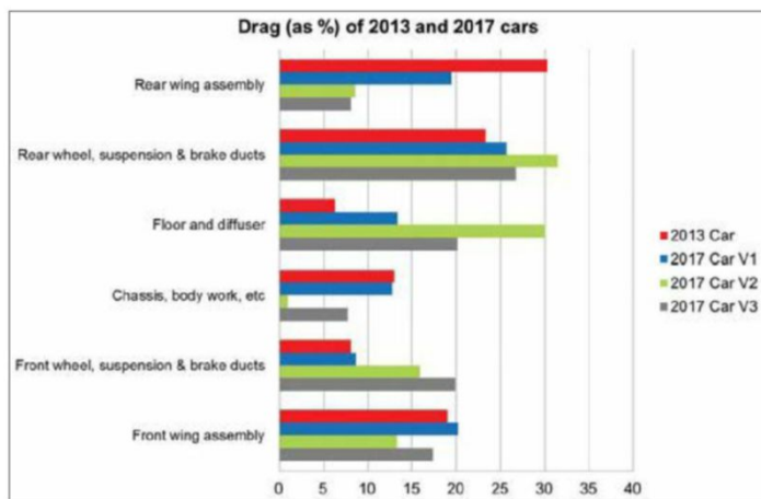
Figure 11: This shows the drag contributions from the major component groups on our cars. Note that the overall drag reduced incrementally from the 2013 car to 2017 V3
