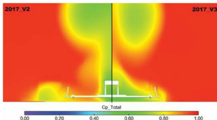
Figure 18: A transverse total pressure slice at the front wing leading edge at four car lengths separation shows that the V3's front wing received less energetic airflow
