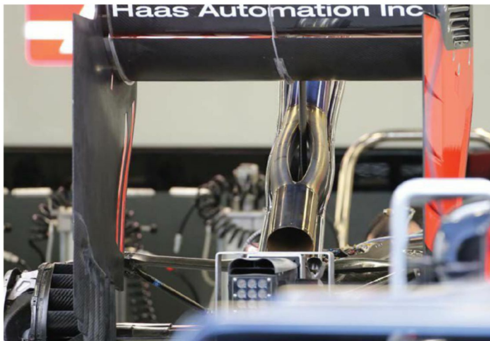
The Haas has the rear wing pylon passing through a split exhaust tail pipe. This is actually a solution pioneered by the Toro Rosso team which is now becoming popular up and down the pit lane. Aero development of VF-16 was done at Maranello
