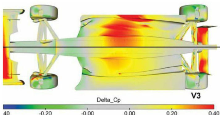
Figure 17: Underside surface pressure changes on the following car at four lengths separation on V2 and V3; note big differences in front wing and underbody responses
