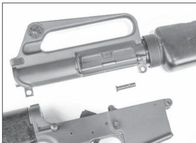
The Colt Model 601 and 602 military rifles used a removable forward pivot pin with a built-in detent. This looks like something that would be easy to lose in the field.
