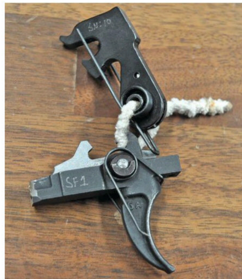
The very first SSF trigger prototype made by hand by Bill Geissele from one of his Hi-Speed triggers for an unnamed elite military unit.
