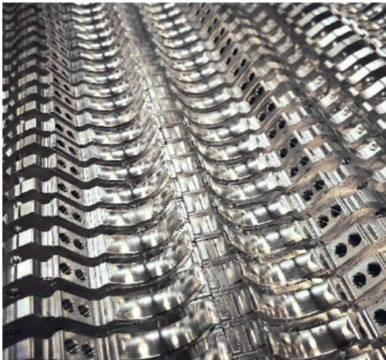
Hundreds of Geissele's new trigger for the Remington 700, in the white.
