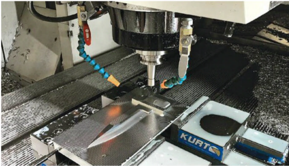
A milling machine hard at work at Abe and Moe knives inside the Geissele factory.
