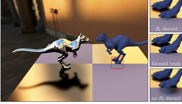
Figure 10: We illustrate the need for our moving occluders bandwidth to discard samples during animations in the KILLEROO scene after 10 frames. Without this bandwidth, the cache incorrectly reproject shadows (bottom inset) onto the screen which result in a dark region in at the feet of the Killeroo.
