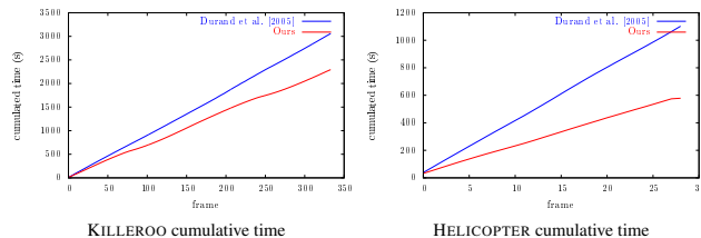
Figure 14: When comparing cumulative rendering times, our cache (in red) allows for smaller rendering time compared to the non-caching method [DHS*05] (in blue) where radiance points are recomputed every frame. In the case of HELICOPTER we achieve almost half the rendering time since we reuse most of the cache samples.
