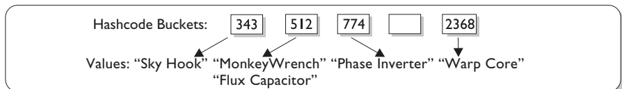
HashMap: The salesman's products (Keys generated from product IDs)
