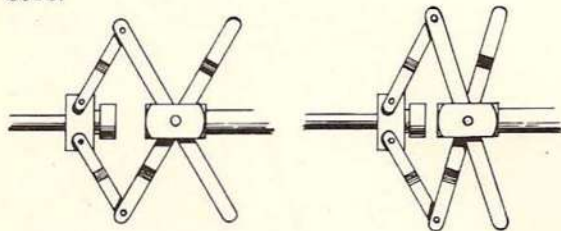
Governor at low speed.
