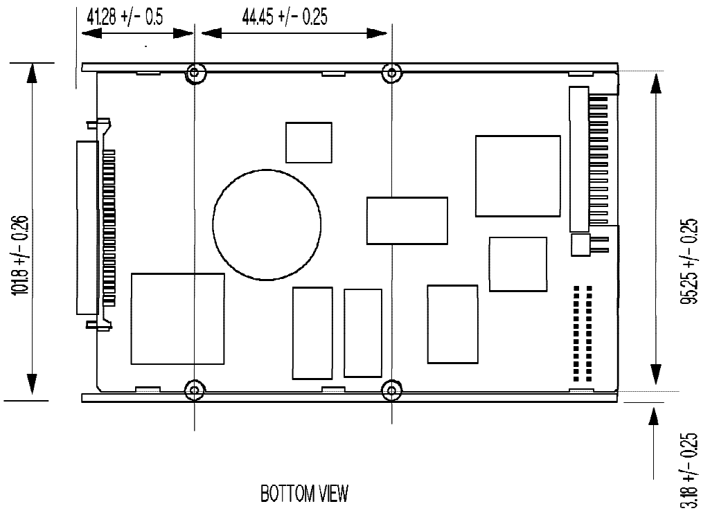
Figure 20. Location of Bottom Mounting Holes for 80 pin SCA-2 models.
