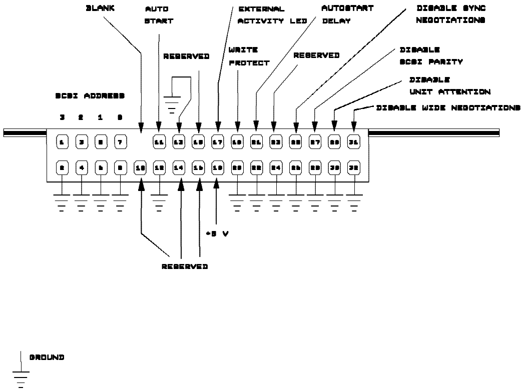
Figure 27. SCA-2 Front Option Jumper Block
