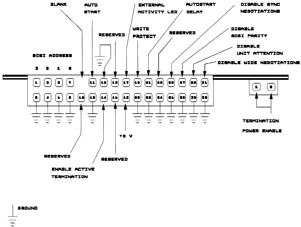
Figure 26. 68 pin Single Ended Front Option Jumper Block and TermPower Block
