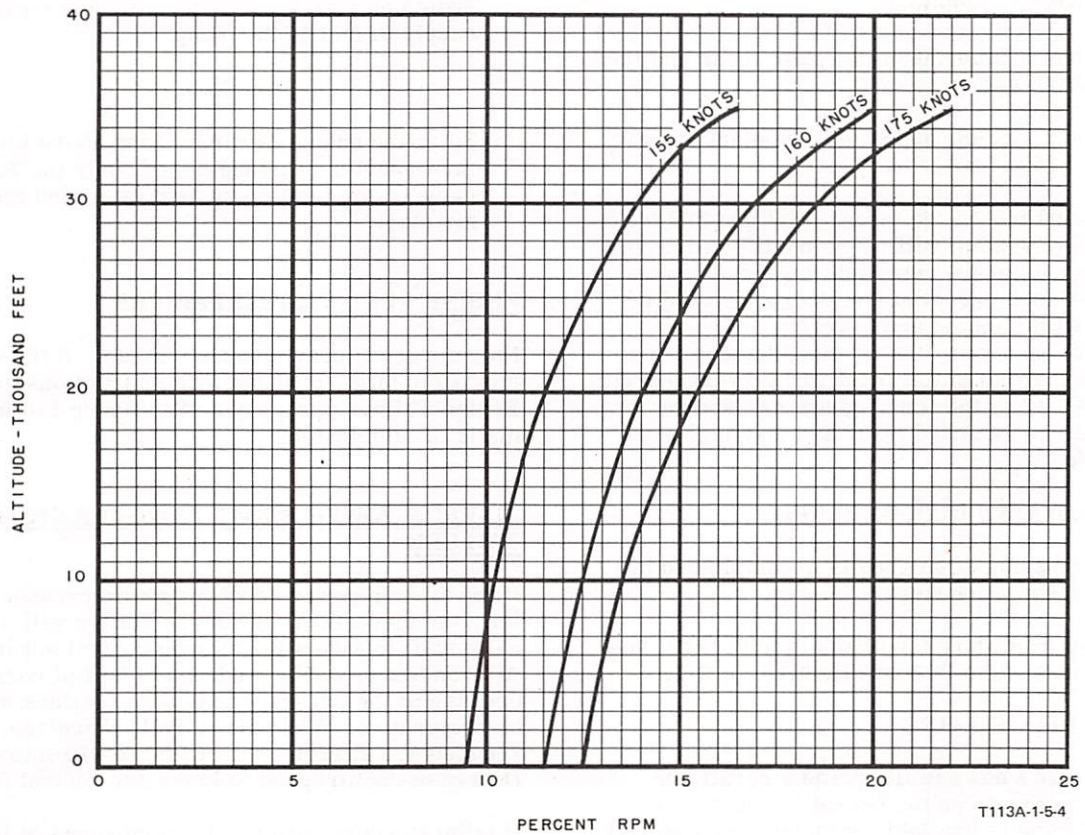
Figure 5-4. Engine Windmill Speed
