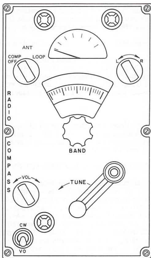
Figure 7-5. Radio Compass Controls (ARN-6)
