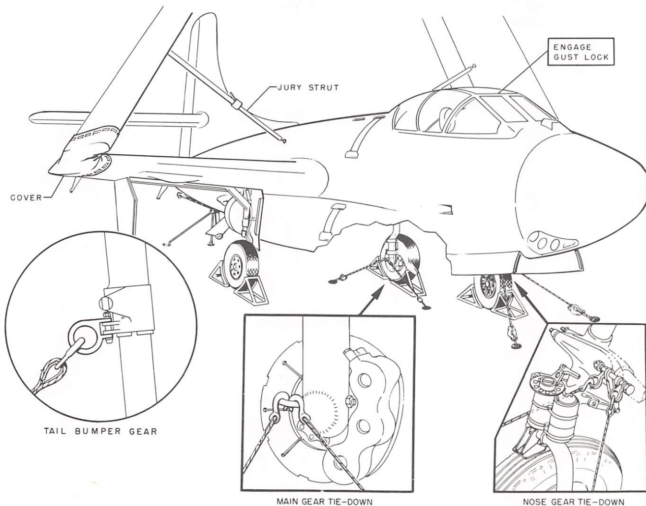
Figure 3-2. Mooring
