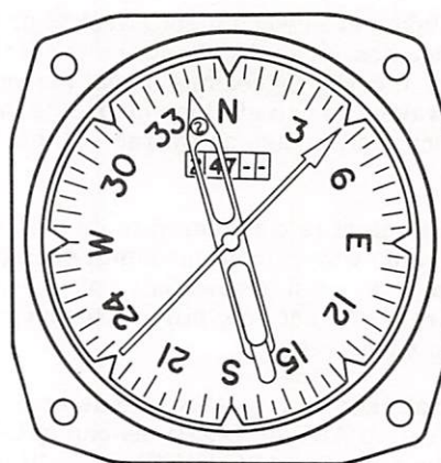
BDHI
