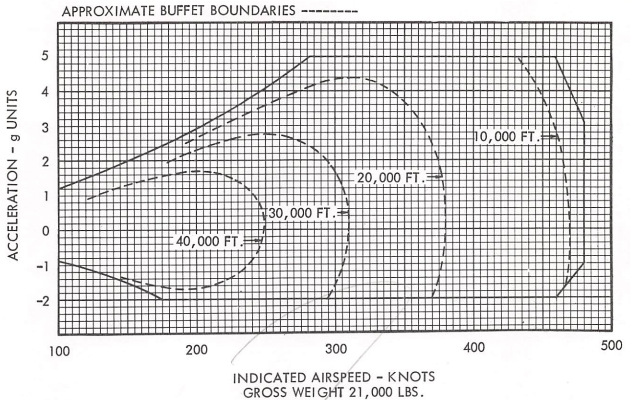
Figure 1-18. Operating Flight Strength Diagram
