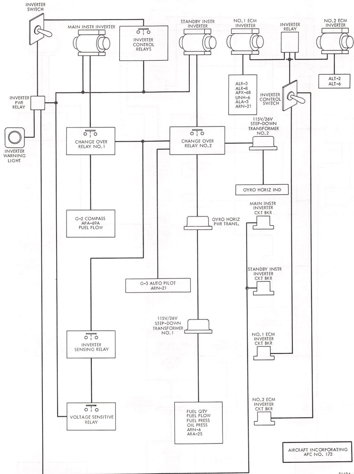
Figure 1-11. AC Electrical System (Sheet 1)
