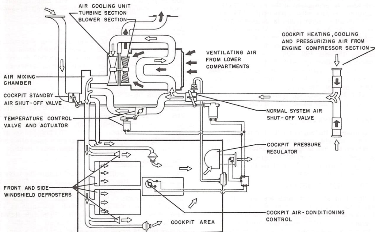
NORMAL AIR CONDITIONING AND PRESSURIZING SYSTEM
