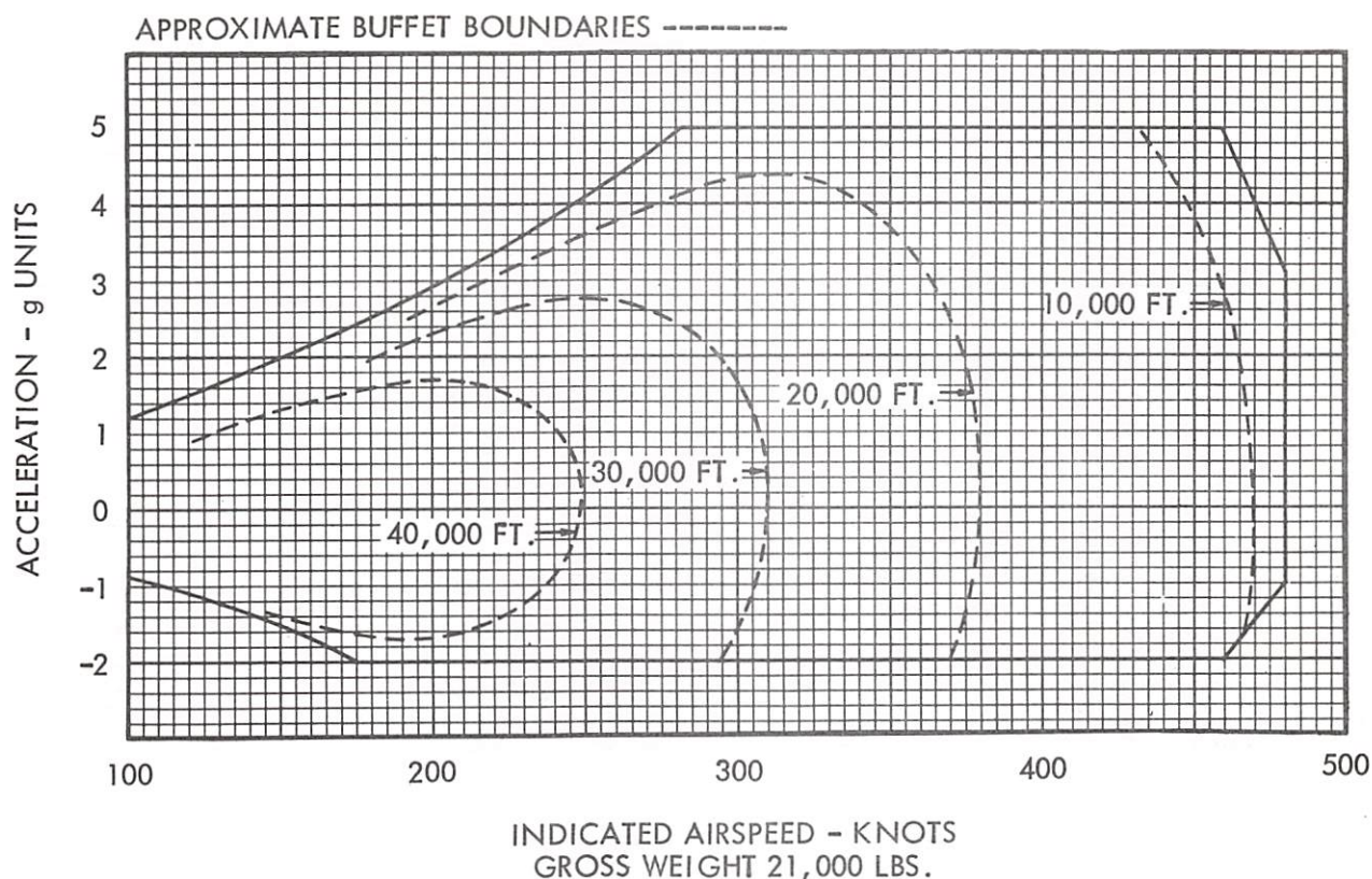
Figure 1-18. Buffet Boundary Operating Flight Strength Diagram ch. 9
