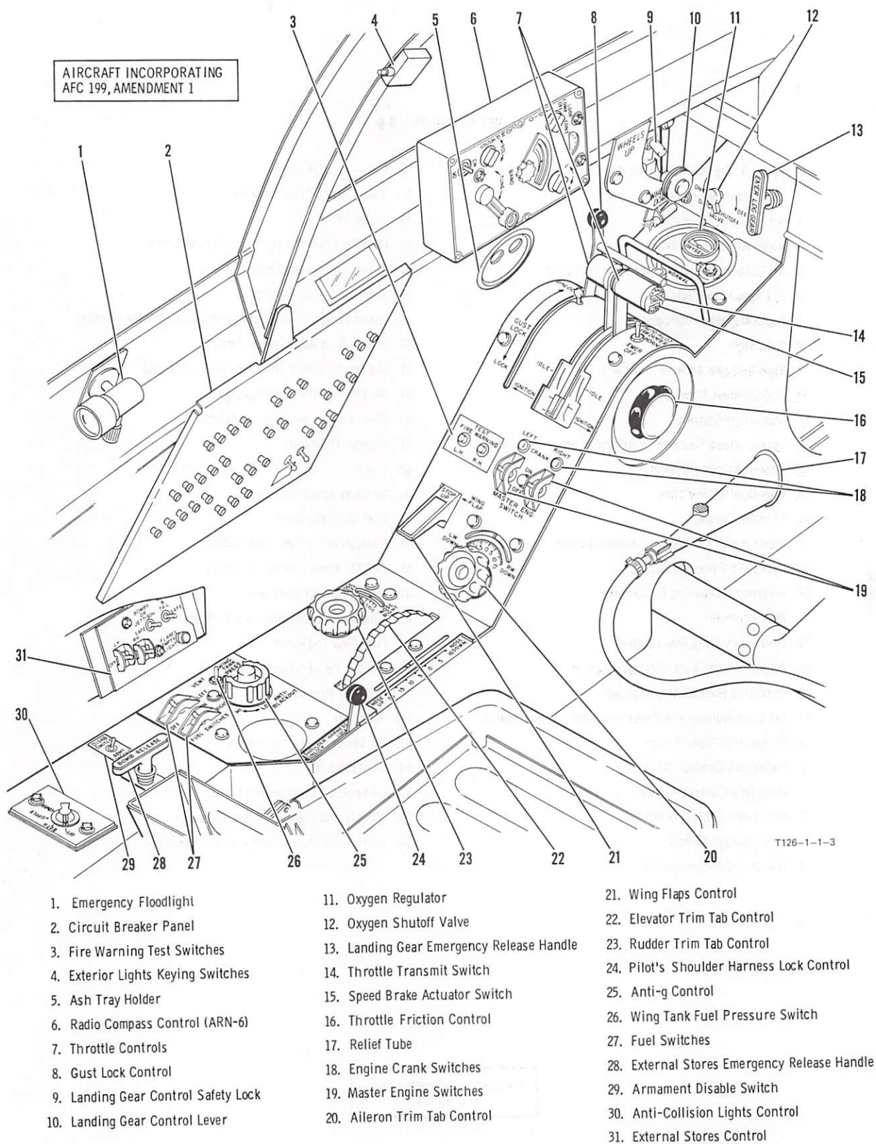
Figure 1-3. Cockpit - Left Side (Sheet 2)
