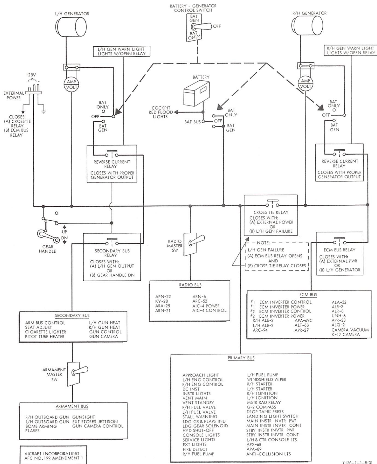
Figure 1-10. DC Electrical System (Sheet 3)
