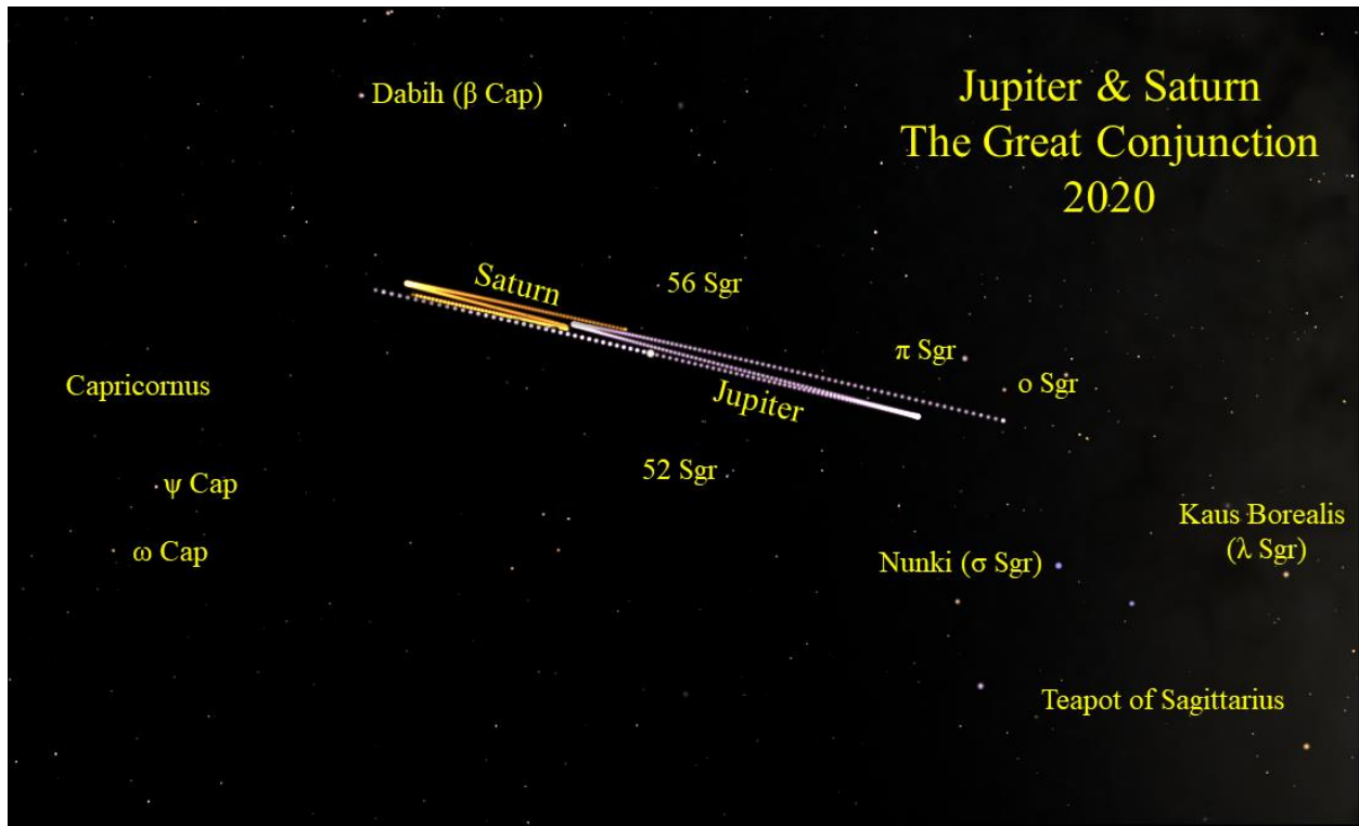
Figure 1 The chart above shows the general celestial regions for the apparitions of the planetary pair among the dim star fields of Sagittarius and Capricornus.
