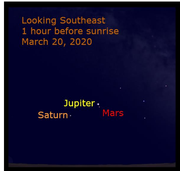
Figure 3 2020, March 20: Mars passes Jupiter in the southeastern morning sky with Saturn nearby.
