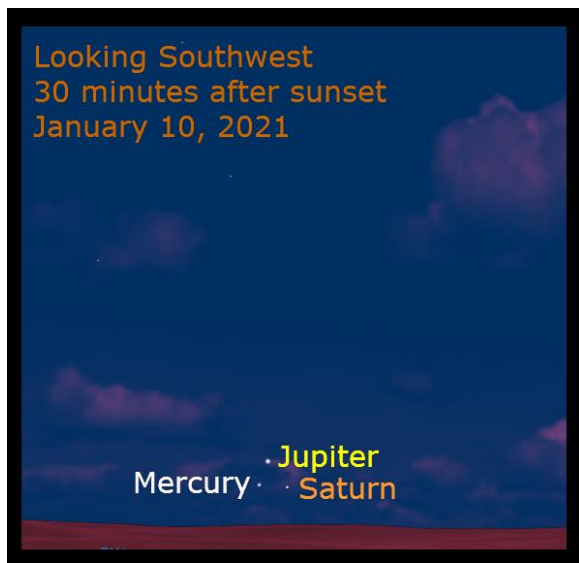
Figure 6 2021, January 10: Mercury joins Jupiter and Saturn in the southwest during bright twilight as the outer planets head toward their solar conjunctions.
