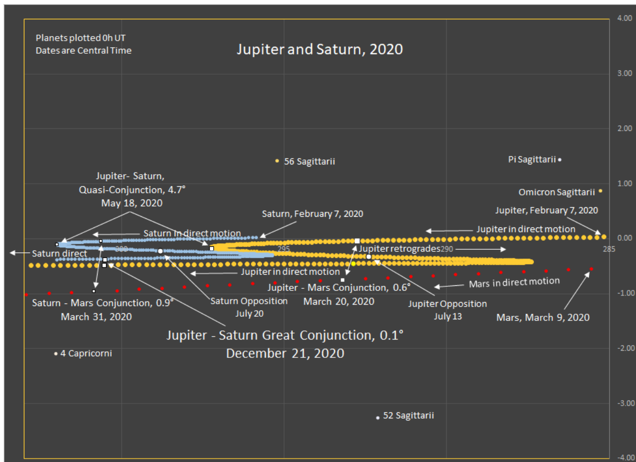
Figure 2 The chart above shows a section of the ecliptic, 18^\circ long, where the planets appear during most of 2020. The planets appear against the background stars of eastern Sagittarius and western Capricornus. The chart includes the path of Mars.
