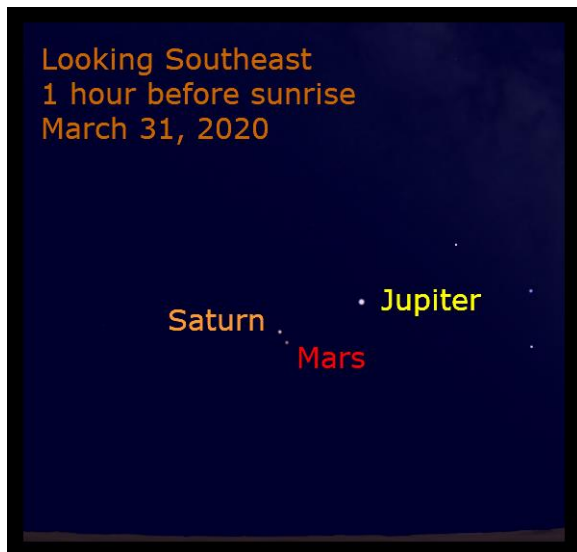
Figure 4 2020, March 31: Look in the southeast for the Saturn – Mars conjunction about an hour before sunrise.
