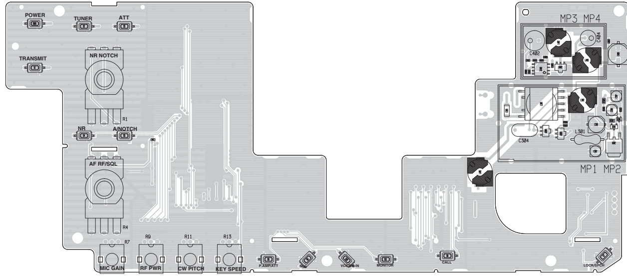
• S-LOGIC UNIT (TOP VIEW)
