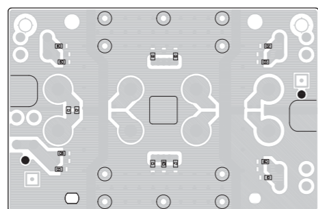
• FILTER BOARD (BOTTOM VIEW)
