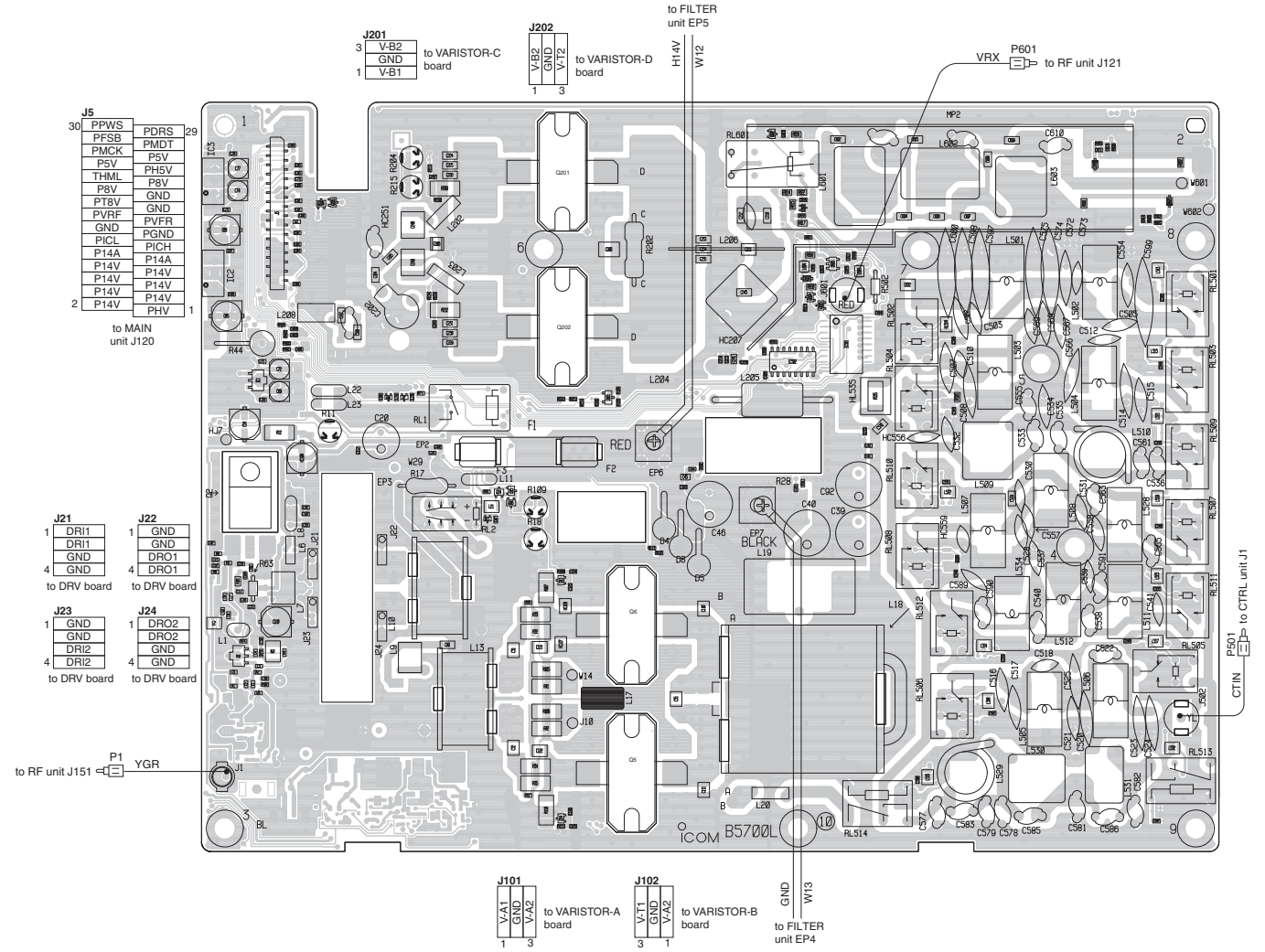
• PA UNIT (TOP VIEW)
