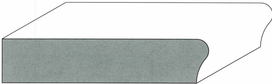
SIL-305 3-1/2 Sill
