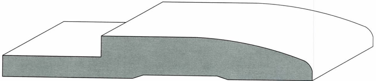
THR-501 5-1/2 Threshold
