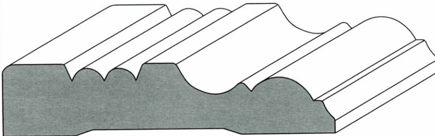
CAS-318 3-1/2 1867 Casing
