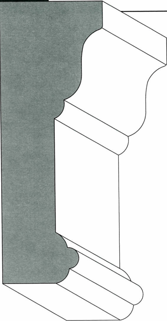
ARC-401 4-3/4 Architrave
