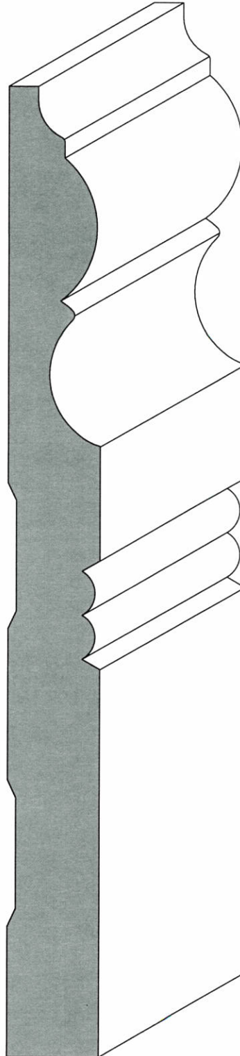
BAS-702 7-1/4 1867 Base
