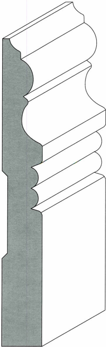
BAS-518 5-1/4 1867 Base
