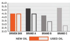
VISCOSITY BREAKDOWN % Viscosity Loss In KRL Shear Test
