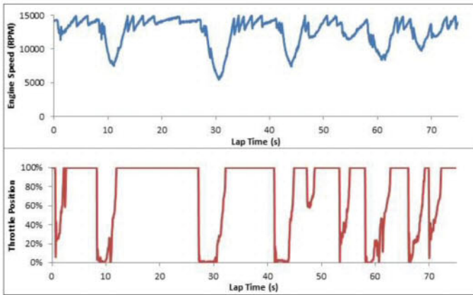
Figure 8: normalised engine speed and throttle position of F1 vehicle at Hockenheim (from Cosworth Electronics, Pi Toolbox, 2009)
