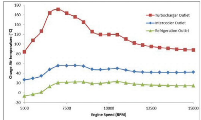
Figure 9: charge air temperature overview
