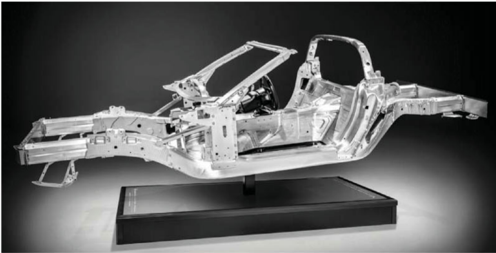
The aluminium frame structure of the Stingray, with 'greater torsional rigidity to improve ride and handling'
