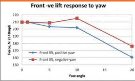
Figure 5: front downforce vs yaw angle
