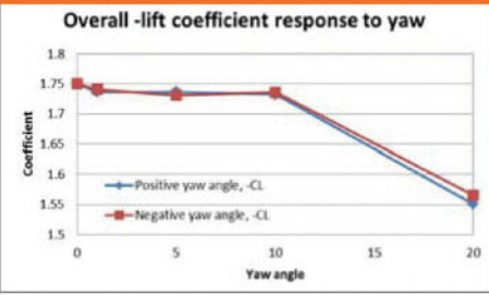
Figure 1: negative lift coefficient vs yaw angle
