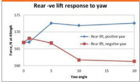
Figure 6: rear downforce vs yaw angle
