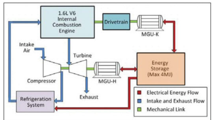
Figure 3: proposed configuration of new engine and related systems
