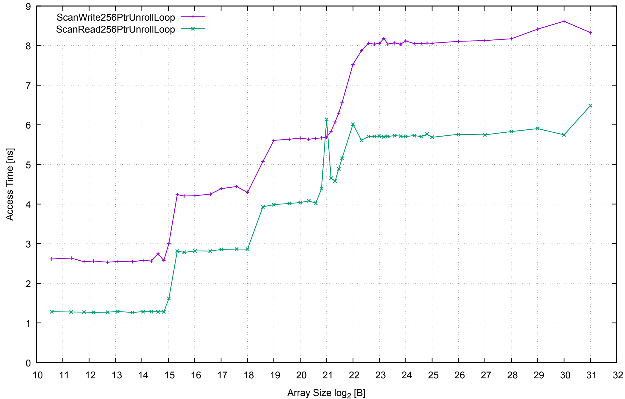
ANDRES-PC - One Thread Memory Latency (excluding Permutation)
