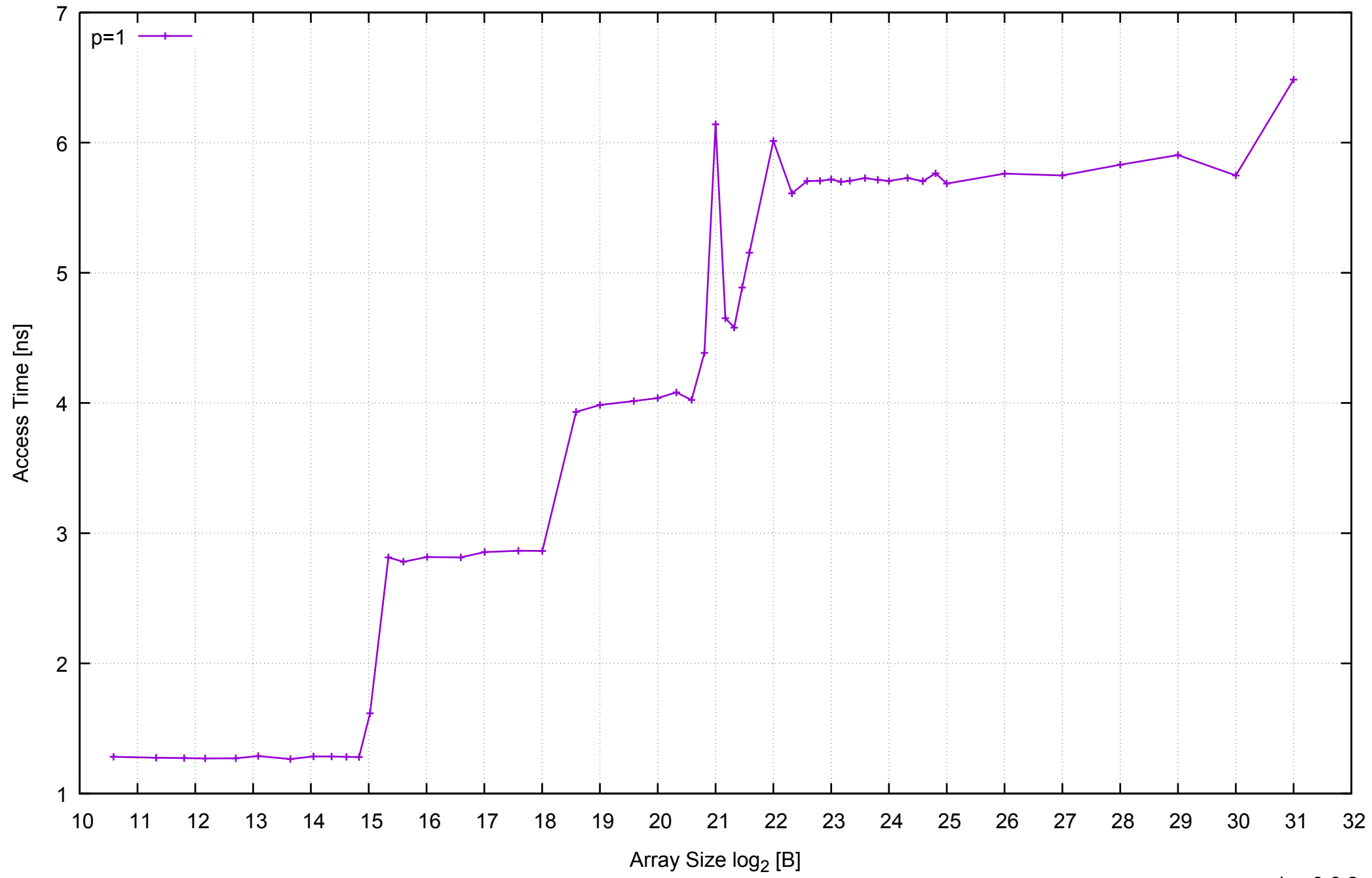
ANDRES-PC - Memory Latency - ScanRead256PtrUnrollLoop
