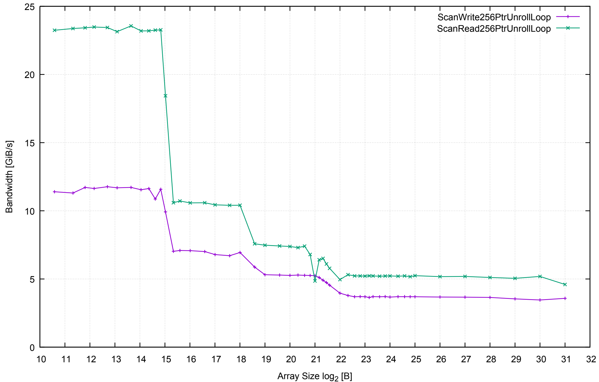
ANDRES-PC - One Thread Memory Bandwidth
