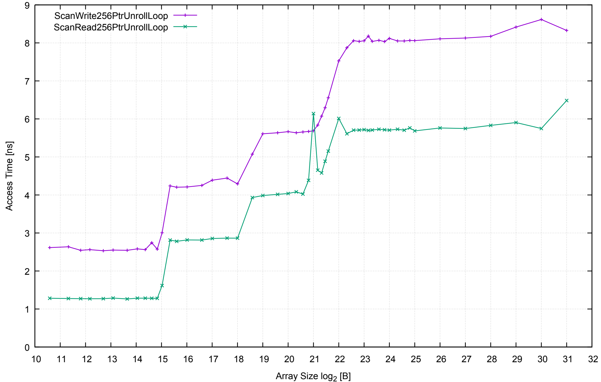
ANDRES-PC - One Thread Memory Latency
