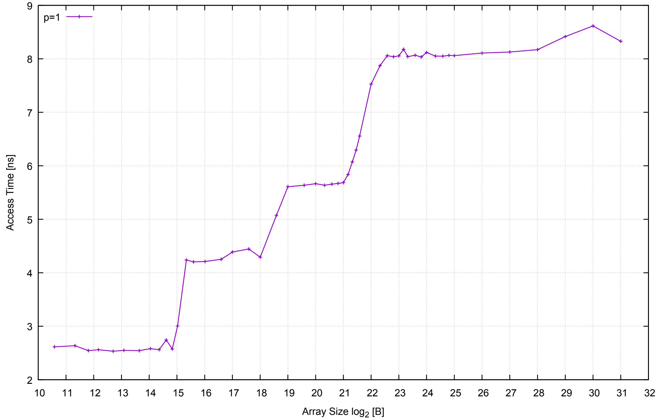
ANDRES-PC - Memory Latency - ScanWrite256PtrUnrollLoop
