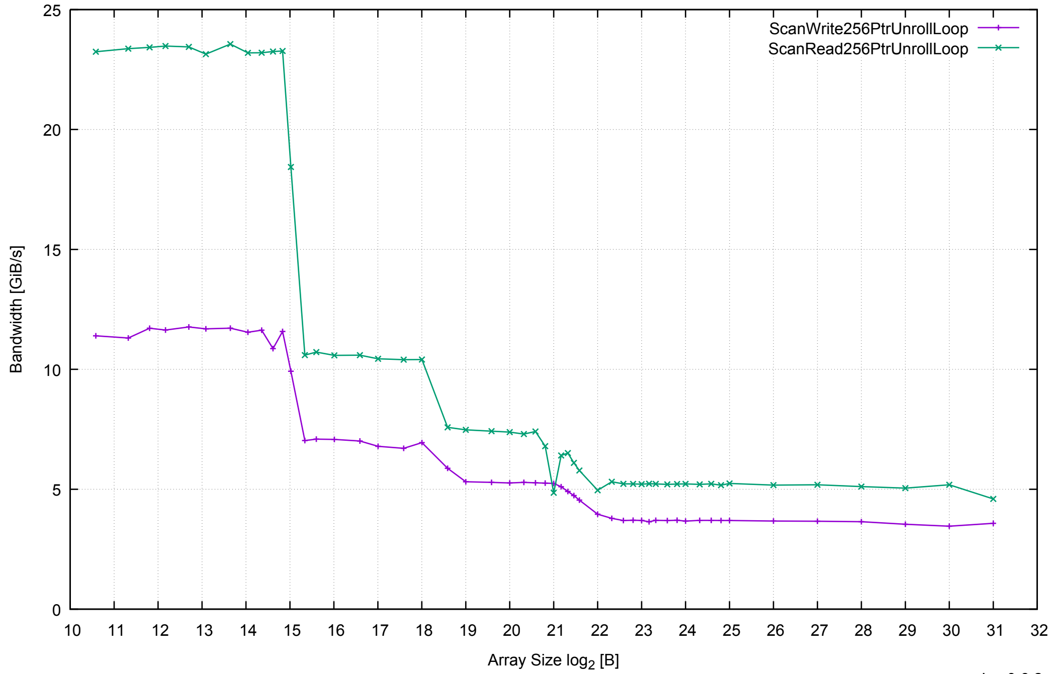
ANDRES-PC - One Thread Memory Bandwidth (only 64-bit Reads)
