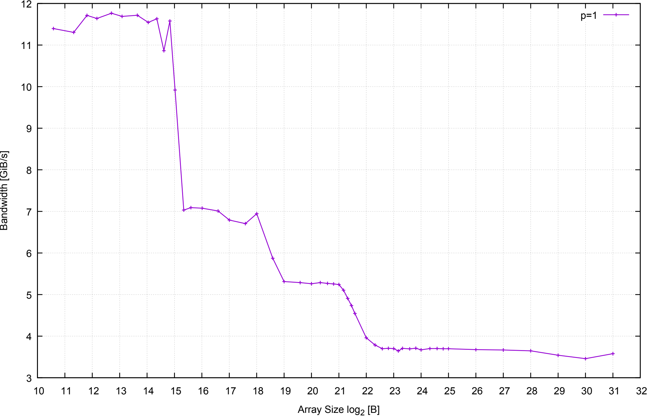
ANDRES-PC - Memory Bandwidth - ScanWrite256PtrUnrollLoop
