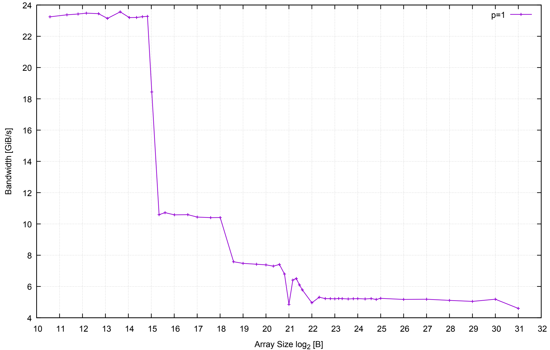
ANDRES-PC - Memory Bandwidth - ScanRead256PtrUnrollLoop
