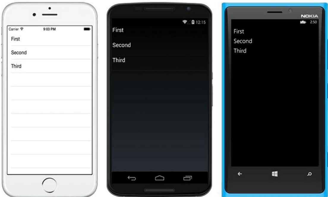
Figure 5-1. ListView in iOS, Android, and Windows Phone
