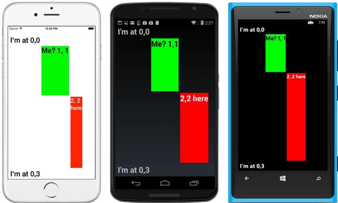
Figure 3-15. Filling available vertical space by using GridUnitType.Star in the Height
