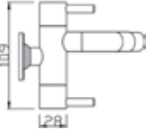
Code : T-72141 Quarter Turn Two-Way Tap
