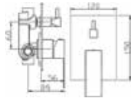
Code : SAM-014-CR Single Lever Concealed Shower Mixer with Diverter * 35mm cartridge
