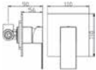
Code : SAM-010-CR Single Lever Concealed Shower Mixer * 35mm cartridge
