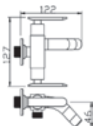
Code : T-84241 Quarter Turn Two-Way Tap
