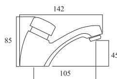
Code : T-1118 Self-Closing Delay Action Tap * 2-4 Litres per min flow rate * 3 second flow duration
