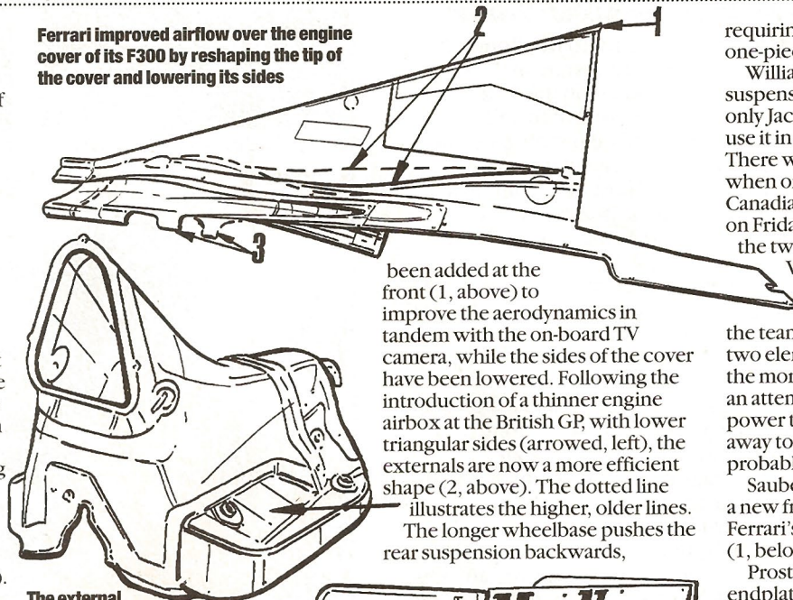
The external dimensions on the Ferrari are more efficient thanks to triangular sides
