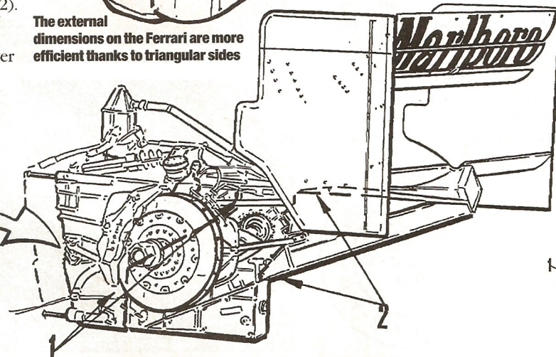
Extra length is gained by increasing size of the spacer between the engine and gearbox
